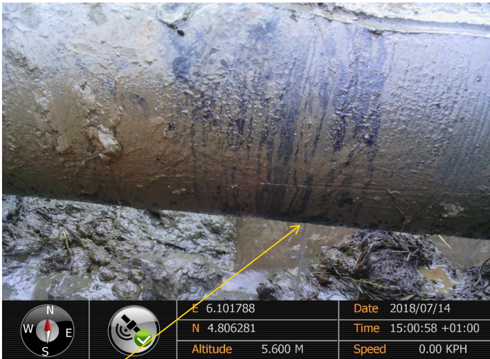
Close-up: Corrosion on 16'' Nun River-Kolocreek Pipeline at Oporoma. Picture was taken during Joint Investigation of 14 th July 2018..
