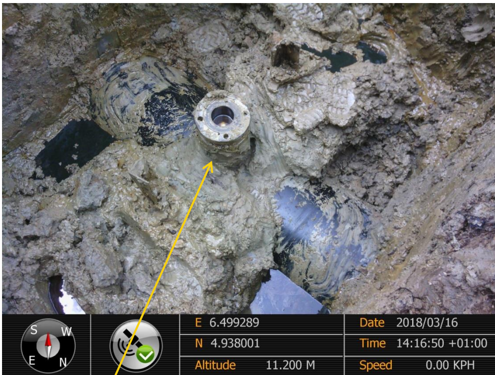
Close-up: Illegal fitting on 20" Kolocreek-Rumuekpe Pipeline at Odau. Picture was taken during Joint Investigation of 16 th March 2018.
