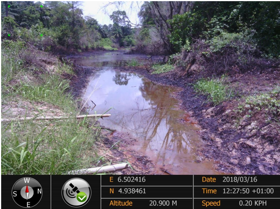
Overview: Part of spill impact on 20" Kolocreek-Rumuekpe Pipeline at Odau. Picture was taken during Joint Investigation of 16 th March 2018.
