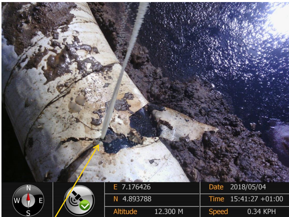
Close-up: Drilled Hole on 12" Imo River-Ogale Pipeline at Umuelechi Uzuaku. Picture was taken during Joint Investigation of 4 th May 2018.
