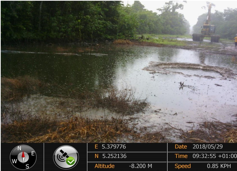
Overview: Part of spill impact on 24" Trans-Ramos Pipeline Right of Way at Odimodi. Picture was taken during Joint Investigation of 29 th May 2018.
