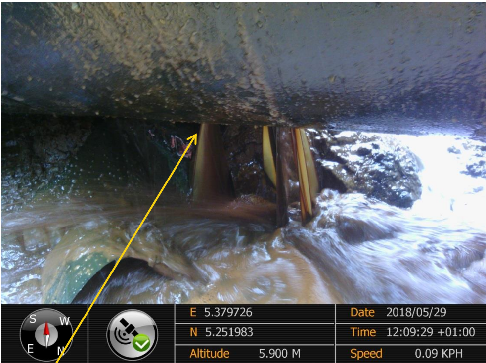
Close-up: Corrosion on 24" Trans-Ramos Pipeline at Odimodi. Picture was taken during Joint Investigation of 29 th May 2018.
