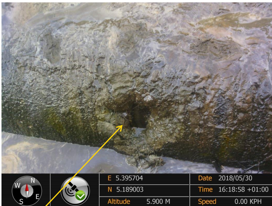
Close-up: Corrosion on 24"Trans-Ramos Pipeline at Odimodi. Picture was taken during Joint Investigation of 30 th May 2018.
