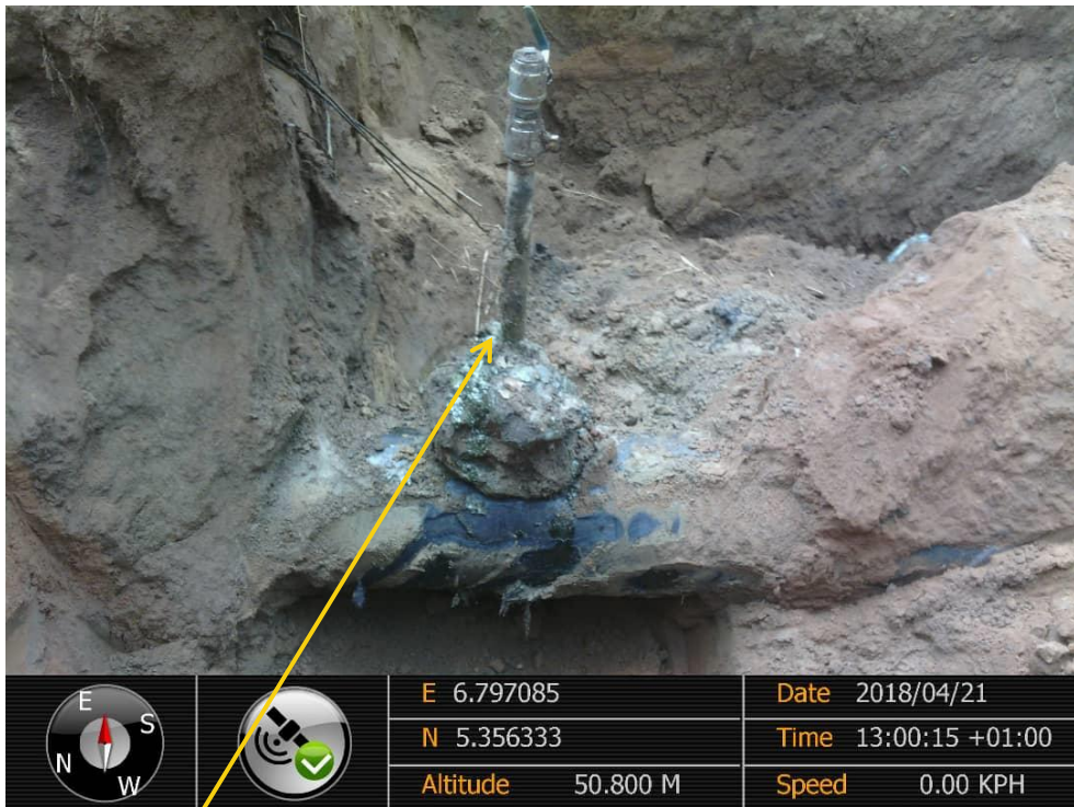
Close-up: Illegal fitting on 18" Assa-Rumuekpe Pipeline at Ochia. Picture was taken during Joint Investigation of 21 st April 2018.
