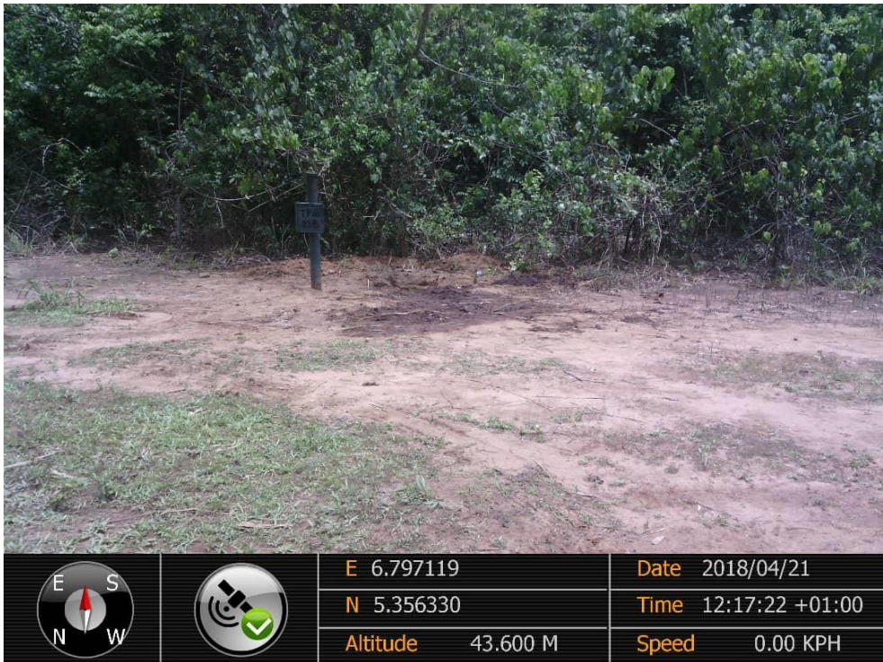
Overview: Part of spill impact on 18" Assa-Rumuekpe Pipeline at Ochia. Picture was taken during Joint Investigation of 21 st April 2018.
