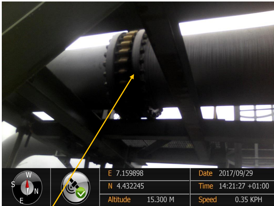
Close-up: Leaking Flange on 01 MOV-411 Filling Valve Flange to Tank 2 at Bonny Terminals. Picture was taken during Joint Investigation of 29 th September 2017.
