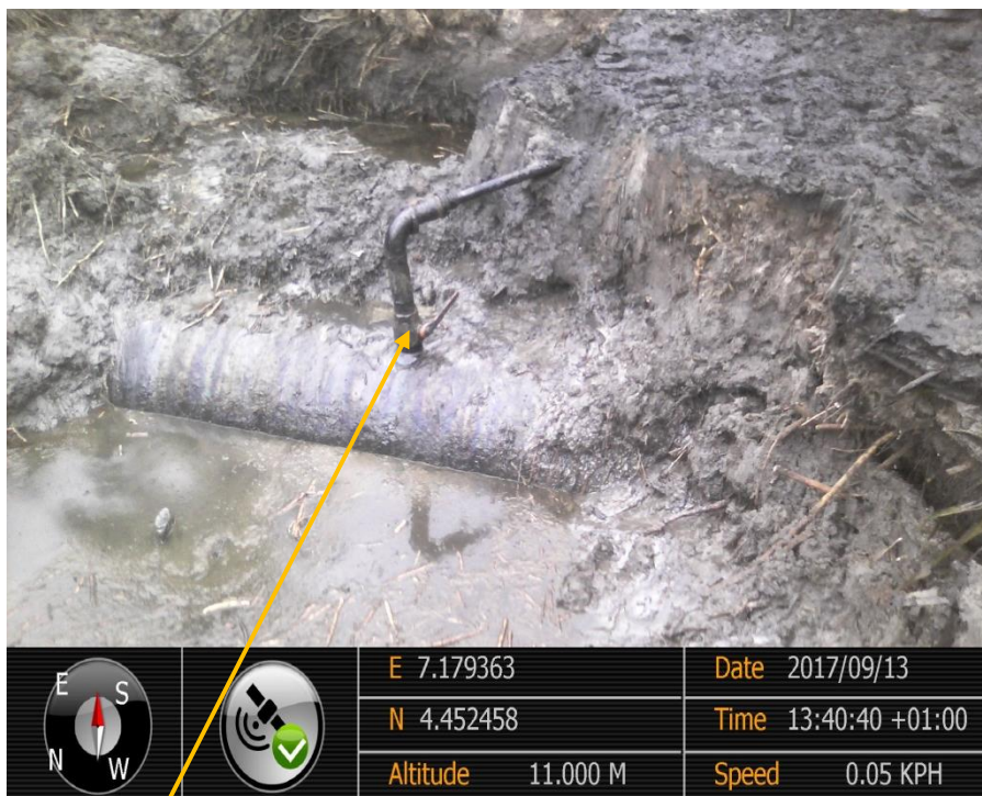
Close-up: Non leaking illegal fitting on 28" Bomu-Bonny Pipeline at Ogbonga Forest Oloma. Picture was taken during Joint Investigation of 13 th September 2017.
