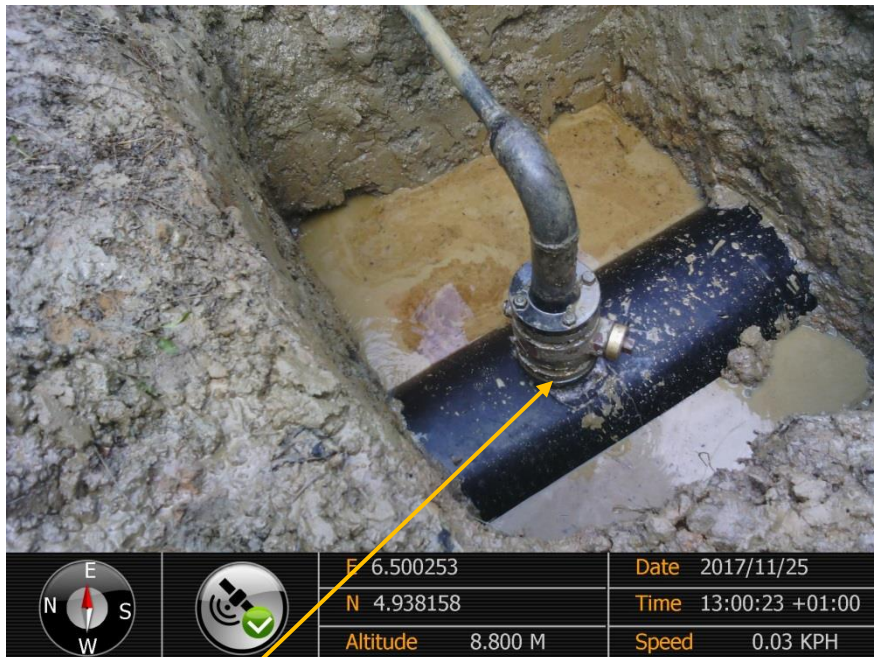
Close-up: Illegal fitting on 20" Kolocreek-Rumuekpe Pipeline at Odau_Ozochi. Picture was taken during Joint Investigation of 25 th November 2017.
