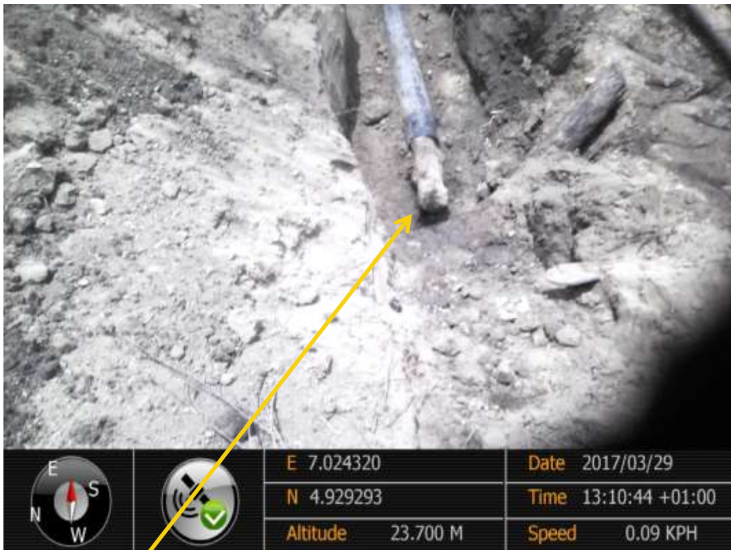
Close-up: Cut section on Agbada 2 Well34S 4" Flowline at Omueke . Picture was taken during initial site visit on 29 th March 2017.
