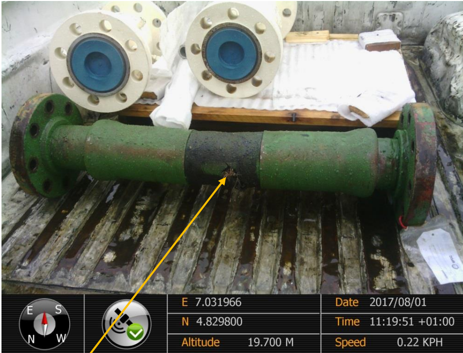
Close-up: Ruptured Flexible Discharge Spool Piece on Belema Flow Station at Belema. Picture was taken during Joint Investigation of 1 st Aug 2017.
