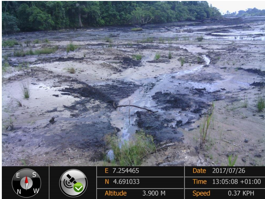
Overview: Part of spill impact on 28" Nkpoku-Bomu Pipeline Right of Way at B-Dere. Picture was taken during Joint Investigation of 26 th July 2017.
