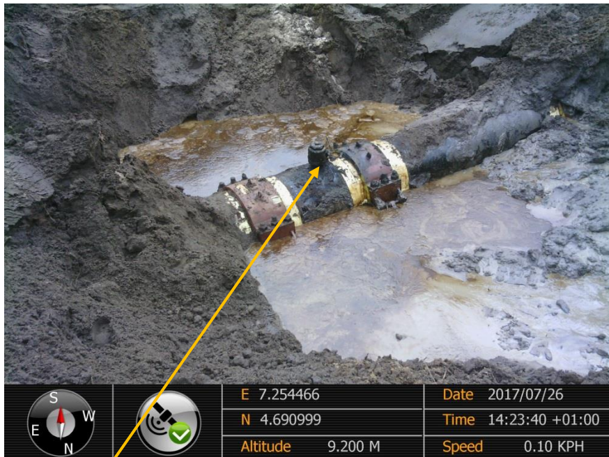
Close-up: Illegal fitting on 28" Nkpoku-Bomu Pipeline at B-Dere. Picture was taken during Joint Investigation of 26 th July 2017.
