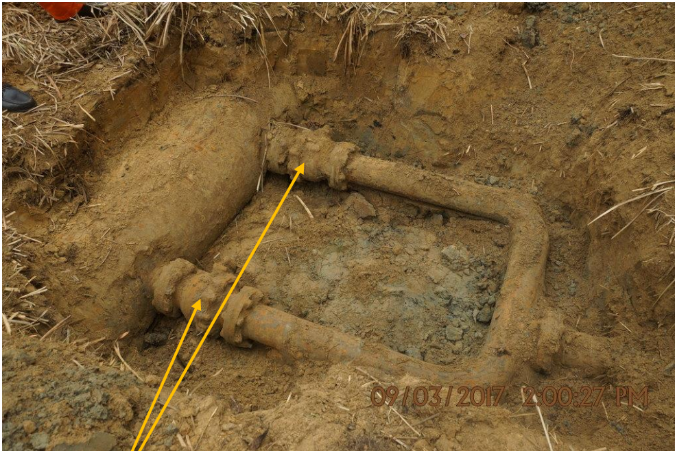
Close-up: 6" valves illegally attached on 24" Trans-Escravos Pipeline at Ogidigben. Picture was taken during Joint Investigation of 9 th March 2017.
