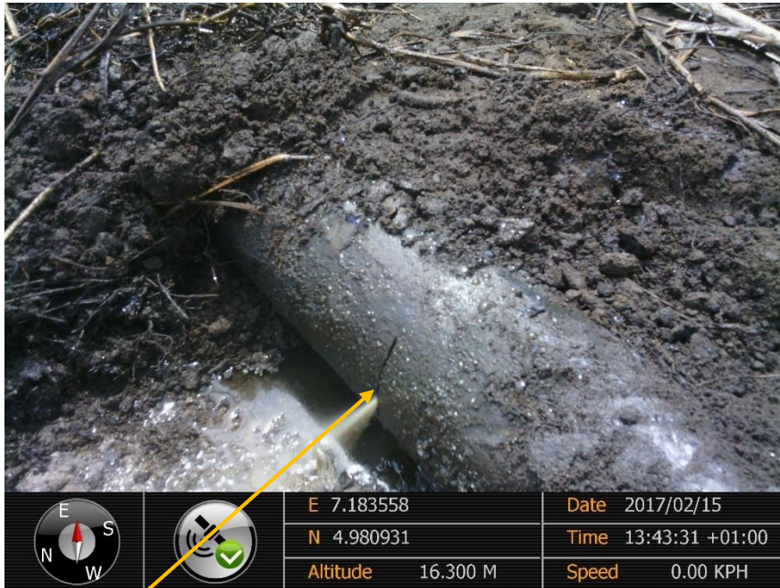
Close-up: Hacksaw cut on Imo River 1 Well 36 Flowline IgiriUkwu-Owaza. Picture was taken during Joint Investigation of 15 th February 2017.
