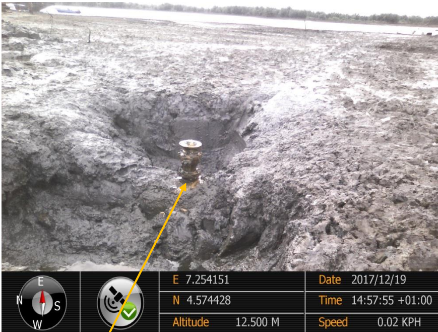
Close-up: Illegal fitting on 28" Bomu-Bonny Pipeline at Patrick Waterside. Picture was taken during Joint Investigation of 19 th December 2017.
