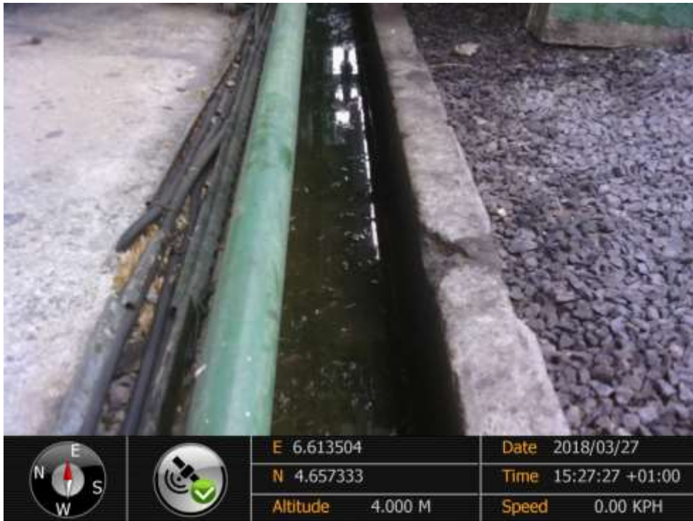
Close-up: Location of observed seepage (Storm Water Drain) at Soku Gas Plant Condensate Spiking pump area at Elem-Sangama. Picture was taken during Joint Investigation of 27 th March 2018.
