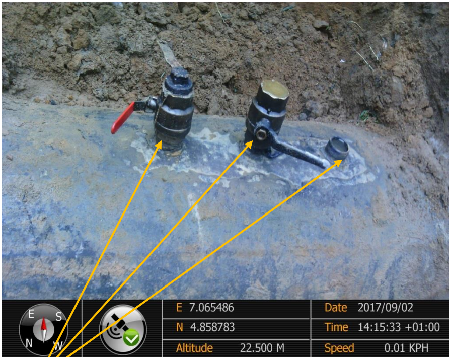
Close-up: Illegal fittings on 28" Nkpoku-Bomu Pipeline at Rumukwurushi. Picture was taken during Joint Investigation of 2 nd September 2017.
