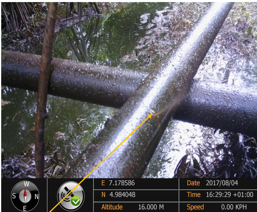
Close-up: Hacksaw Cut on Imo River 1 Well 5S Flowline at Igiriukwu. Picture was taken during Joint Investigation of 4 th Aug 2017.
