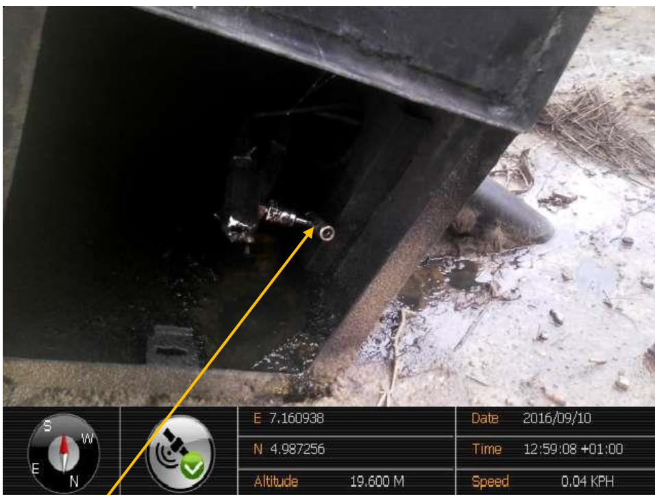
Close-up: Tampered Kerotest Valve on 8" Nkali-Imo River 2 Pipeline (Breathing Tube Box) at Umuedu-Okwara. Picture was taken during Joint Investigation of 10 th September 2016.
