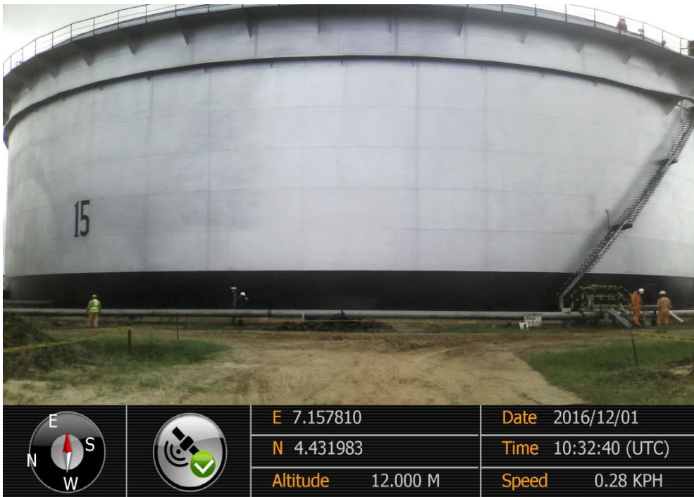
Overview: Part of spill impact on Bonny Terminal tank15-10'' drainline flange at Bonny. Picture was taken during Joint Investigation of 1 st December 2016.
