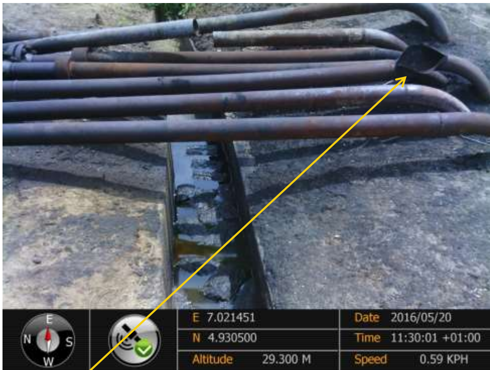
Close-up: Damaged Flowline on Agbada2 Well 41/42/43 Cluster at Omuohia/Omuokoji. Picture was taken during Joint Investigation of 20 th May 2016.
