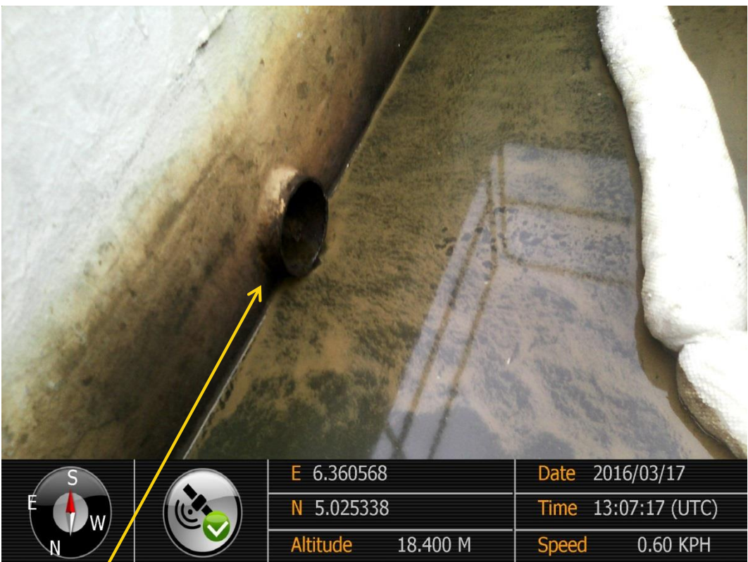
Close-up: Source of leak on Etelebou Flow Station at Ogboloma. Picture was taken during Joint Investigation of 17 th March 2016.
