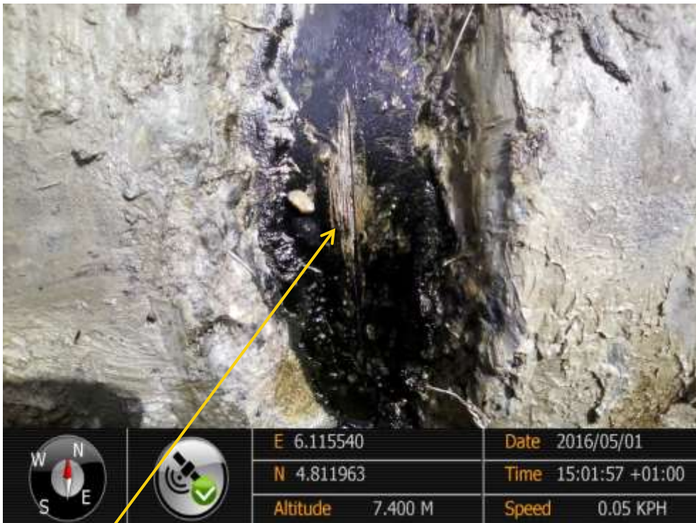
Close-up: Hacksaw cut on 16" Nun River – KoloCreek Pipeline at Oporoma. Picture was taken during Joint Investigation of 1 st May 2016.
