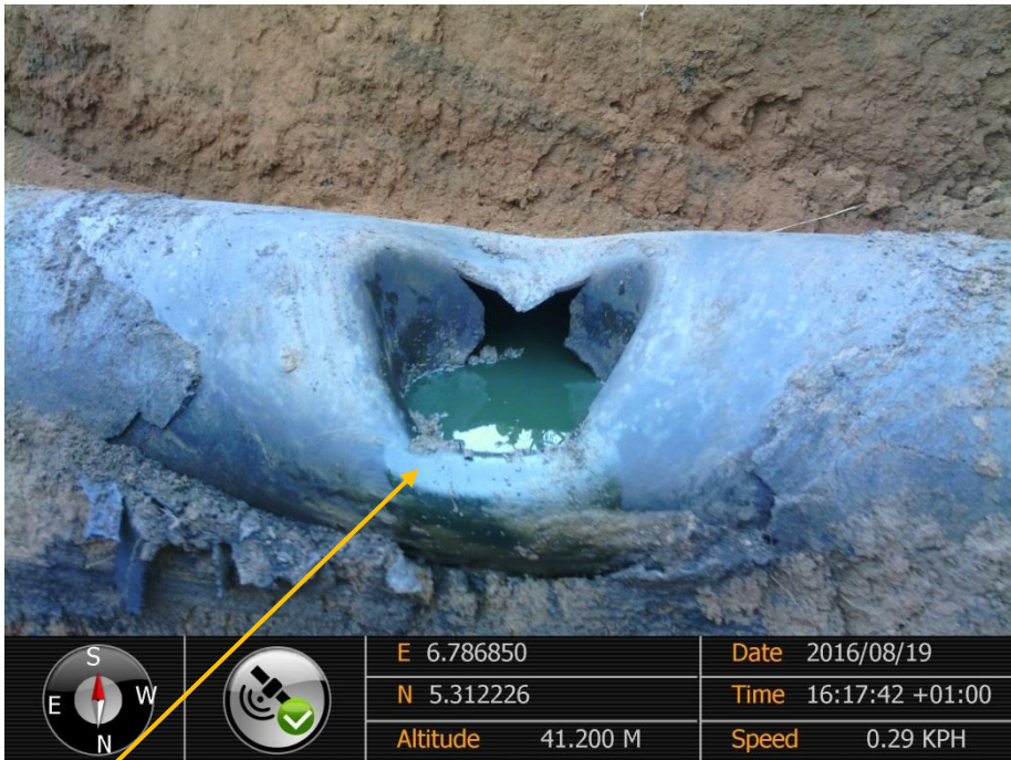
Close-up: Tear/inward dent on 18" Assa-Rumuekpe Pipeline at Ochia. Picture was taken during Joint Investigation of 19 th August 2016.
