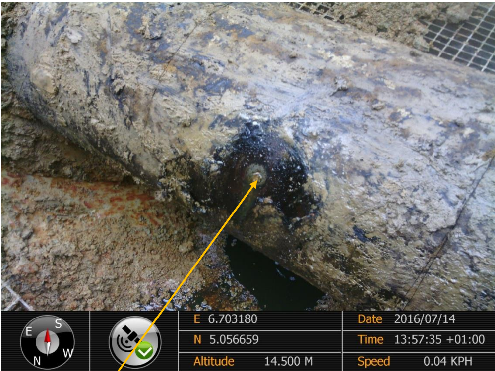
Close-up: Drilled Hole on 18" Assa-Rumuekpe Pipeline at Elele-Alimini Ihuaba. Picture was taken during Joint Investigation of 14 th July 2016.
