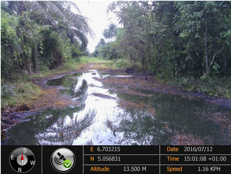
Overview: Part of spill impact 18" Assa-Rumuekpe Pipeline at Elele-Alimini Ihuaba. Picture was taken during Joint Investigation of 12 th July 2016.
