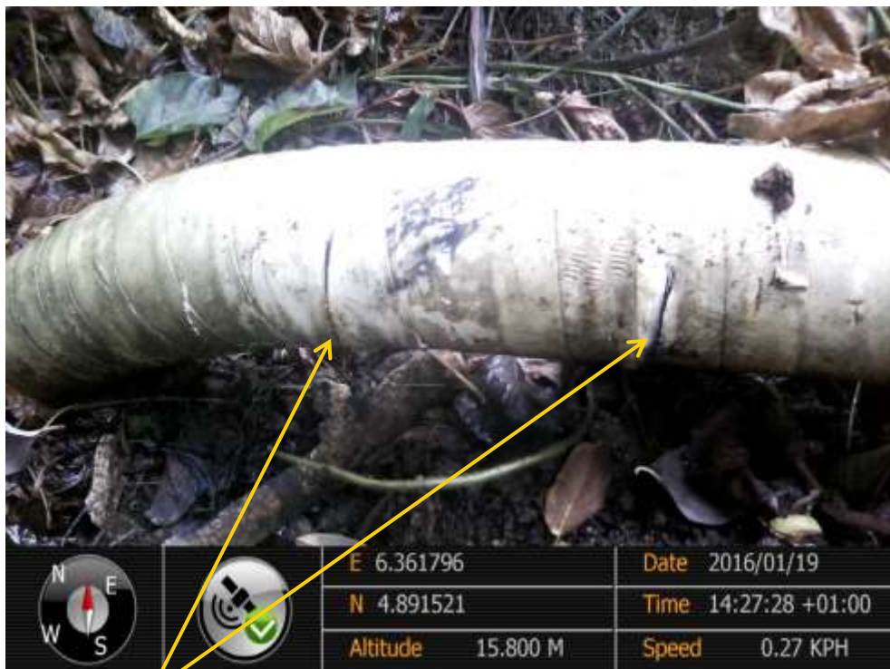
Close-up: Hacksaw cut on KoloCreek Well3T Flowline at Otusega. Picture was taken during Joint Investigation of 19 th January 2016.
