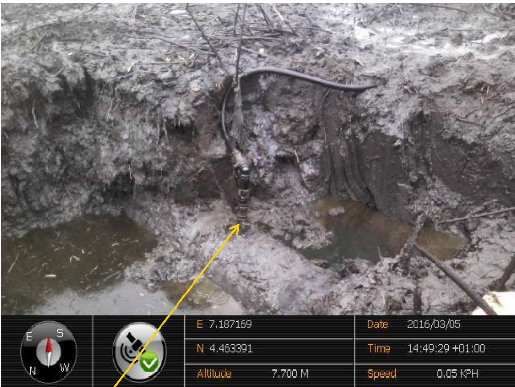
Close-up: Illegal fitting on 28" Bomu-Bonny Trans Niger Pipeline at Anyaminima/Oloma. Picture was taken during Joint Investigation of 5 th March 2016.
