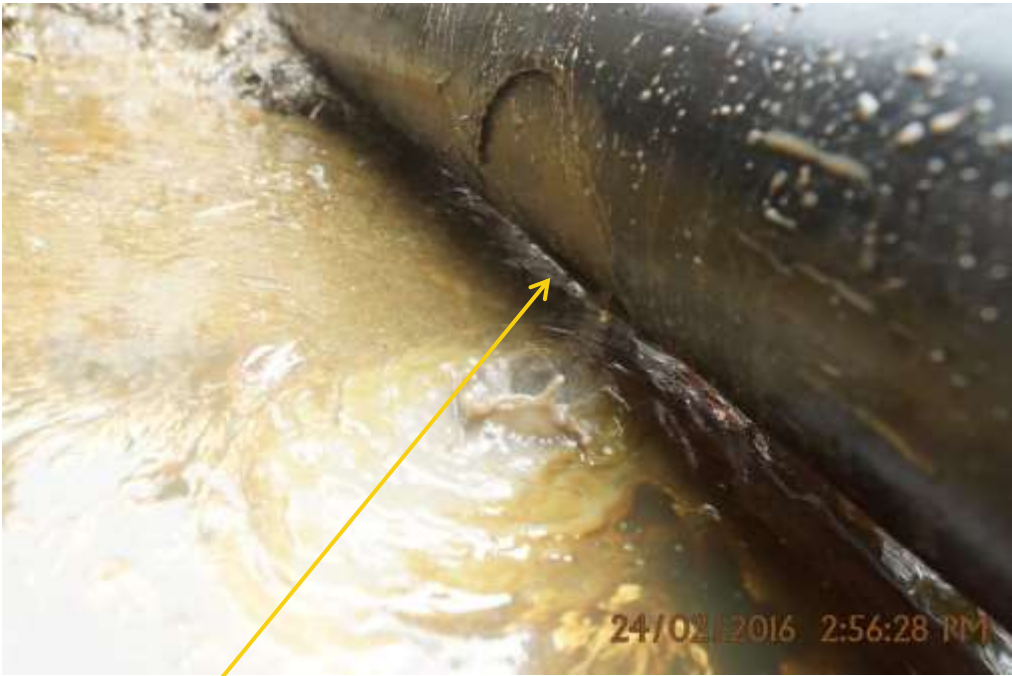
Close-up: 3mm hole on 6" Seibou Bulkline2 at Azagbene. Picture was taken during Joint Investigation of 24 th February 2016.
