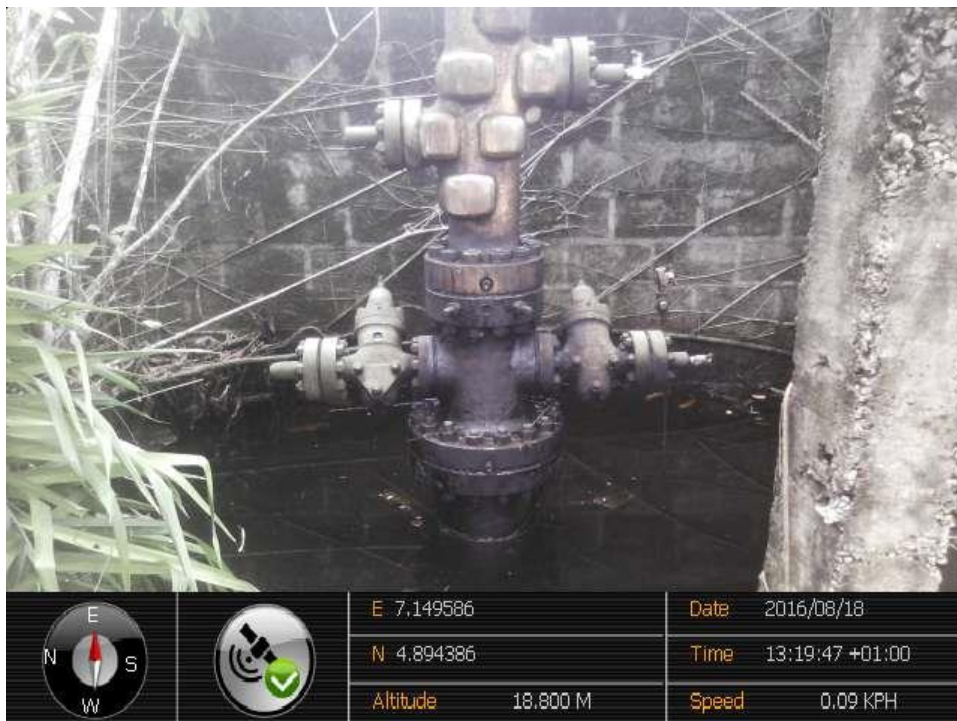
Close-up: Non leaking Obigbo North Well 12 Wellhead at Uzuaku. Picture was taken during Joint Investigation of 18 th August 2016.
