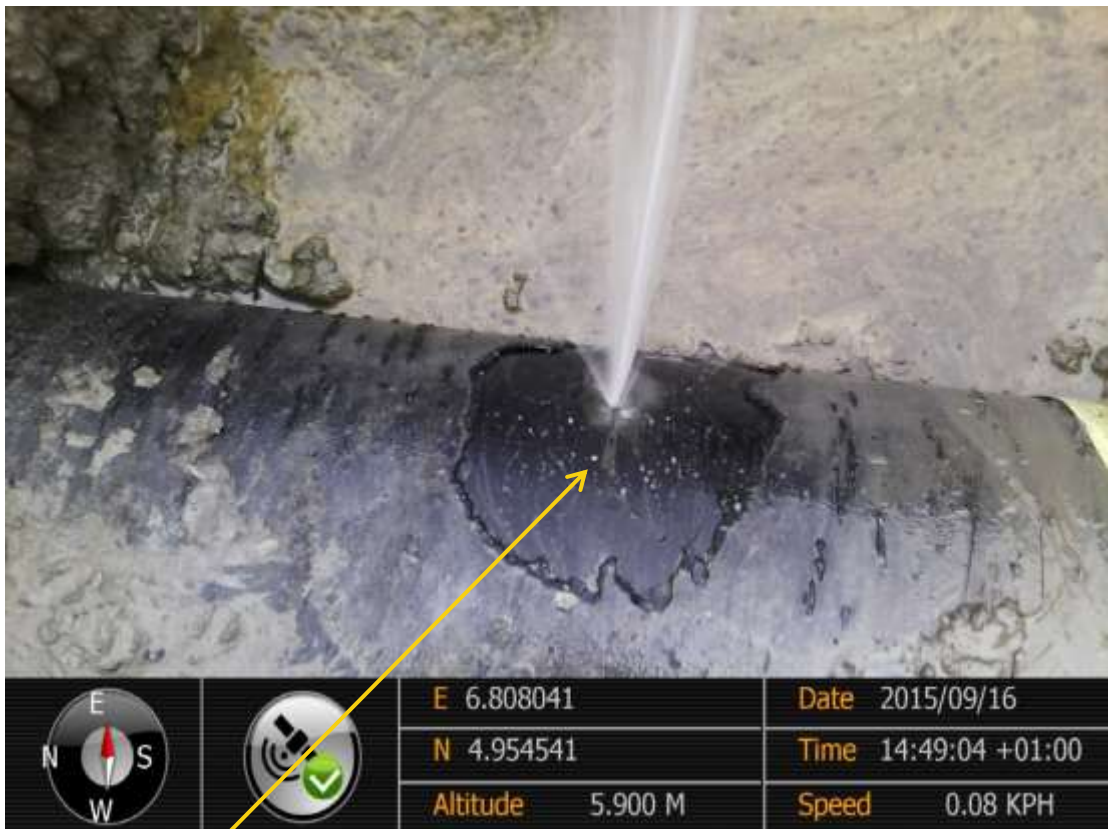
Close-up: Hacksaw cut on 20" Rumuekpe-Nkpoku Pipeline at Omukpobu. Picture was taken during Joint Investigation of 16 th September 2015.
