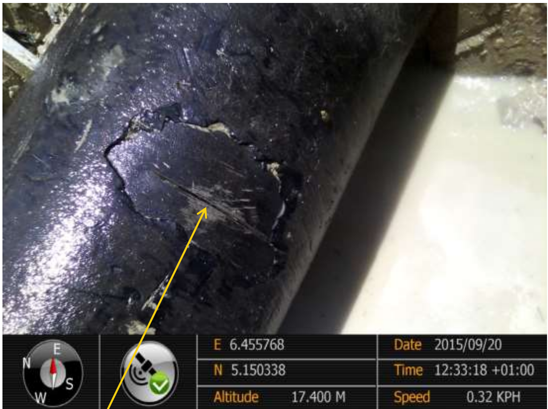
Close-up: Hacksaw cut on 14" Okordia – Rumuekpe Pipeline at Ikarama. Picture was taken during Joint Investigation of 20 th September 2015.
