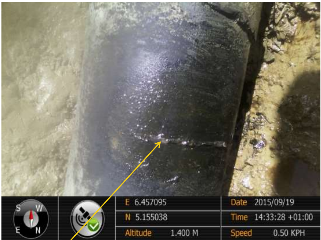
Close-up: Hacksaw cut on 12" Adibawa – Okordia Pipeline at Ikarama. Picture was taken during Joint Investigation of 19 th September 2015.
