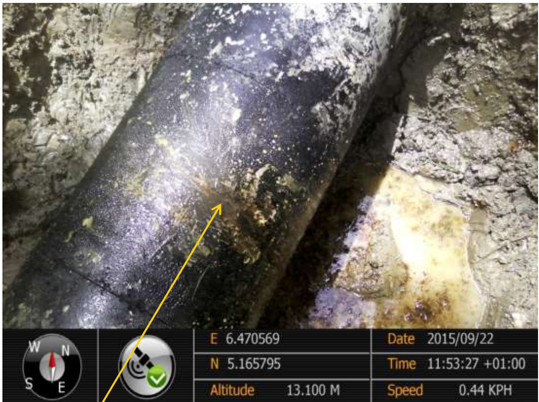
Close-up: Hacksaw cut on 12" Adibawa – Okordia Pipeline at Ikarama. Picture was taken during Joint Investigation of 22 nd September 2015.
