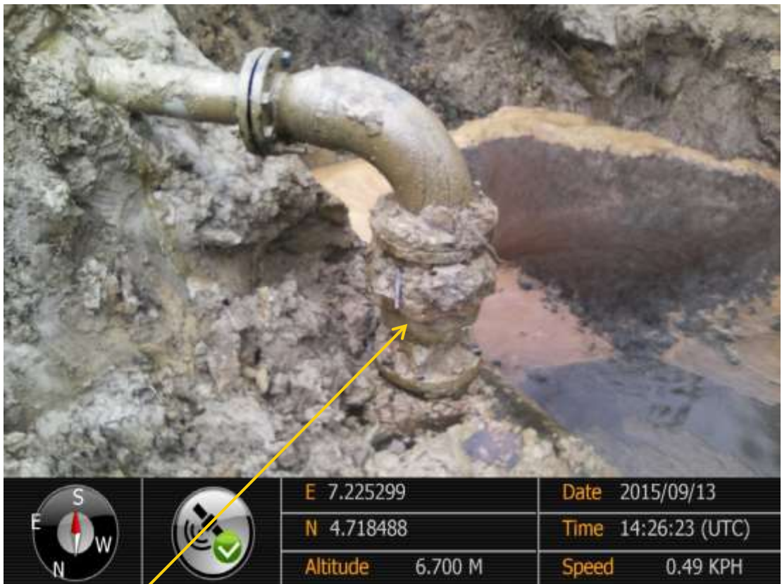
Close-up: Illegal fitting on 28" Nkpoku – Bomu Pipeline at Kporghor. Picture was taken during Joint Investigation of 13 th September 2015.
