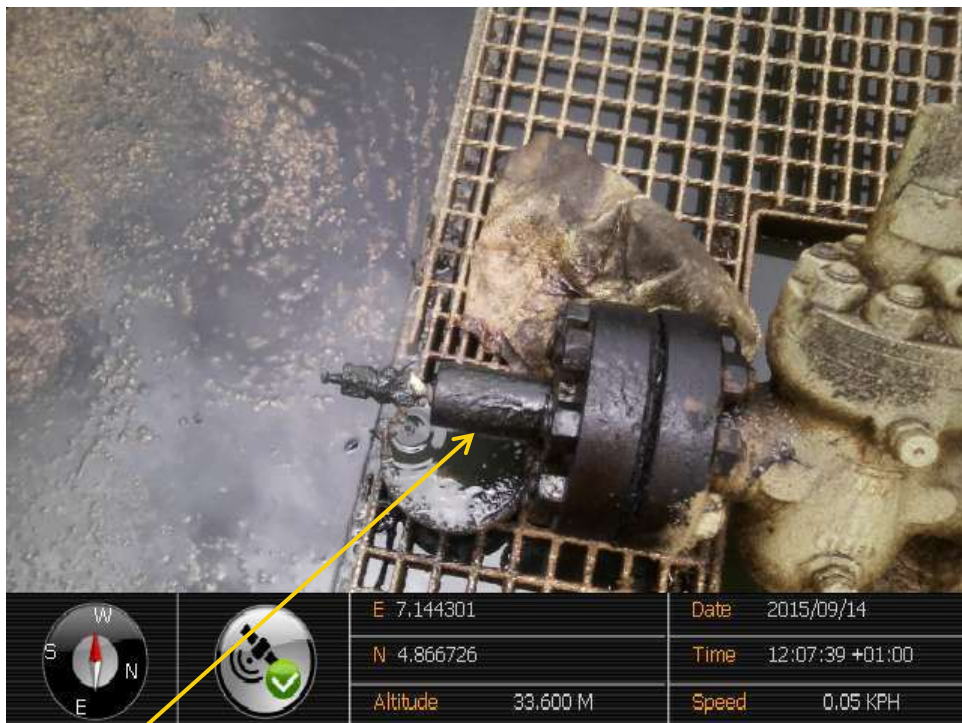
Close-up: Leak due to corrosion on Kerotex Needle valve at Obigbo South Well3L Wellhead at Umusia. Picture was taken during Joint Investigation of 14 th September 2015.
