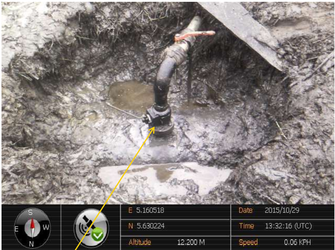
Close-up: Illegal fitting on 20" Otumara – Escravos Pipeline at Ugboegungun. Picture was taken during Joint Investigation of 29 th October 2015.
