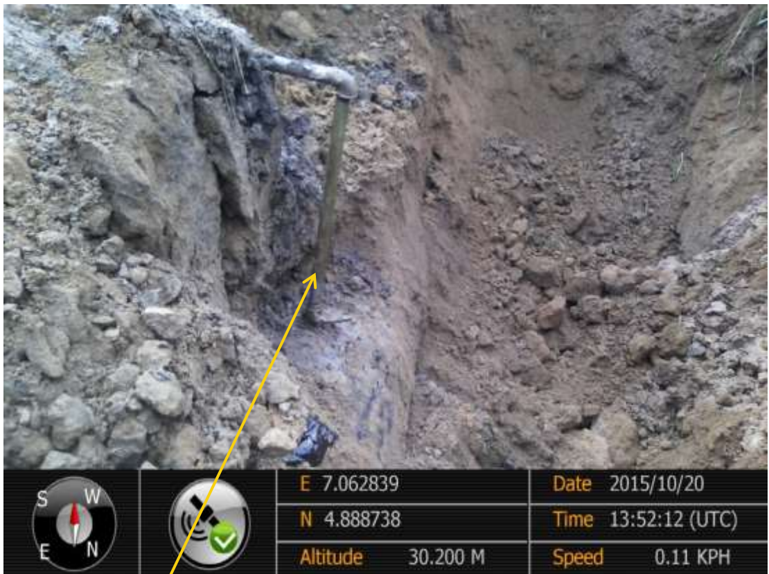
Close-up: Illegal fitting on 36" Nkpoku-Bomu Pipeline at Atali. Picture was taken during Joint Investigation of 20 th October 2015.
