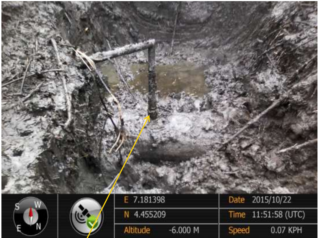
Close-up: Illegal fitting on 28" Bomu-Bonny Trans Niger Pipeline at Anyaminima/Oloma. Picture was taken during Joint Investigation of 22 nd October 2015.
