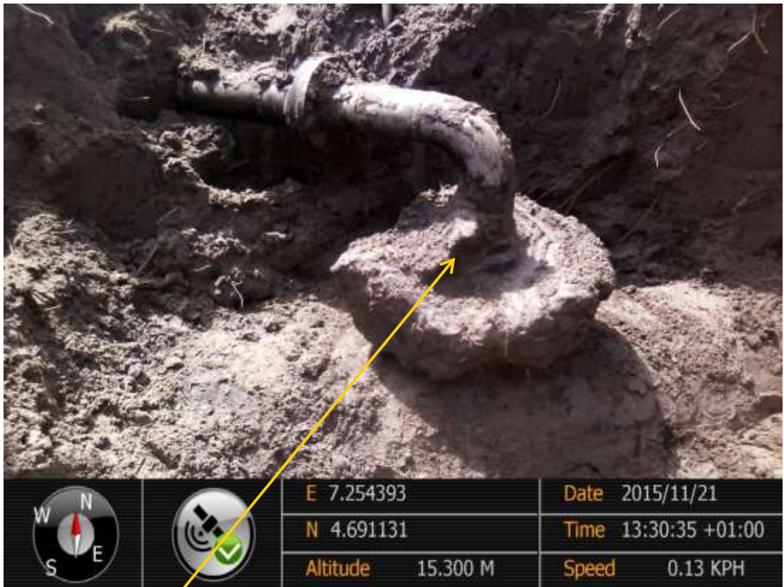
Close-up: Illegal fitting enclosed with concrete on 28" Nkpoku-Bomu Pipeline at B-Dere. Picture was taken during Joint Investigation of 21 st November 2015.
