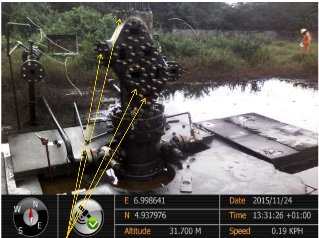
Close-up: Former position of mutiple valves removed from Agbada1 Well50 at Omuchi. Picture was taken during Joint Investigation of 24 th November 2015.
