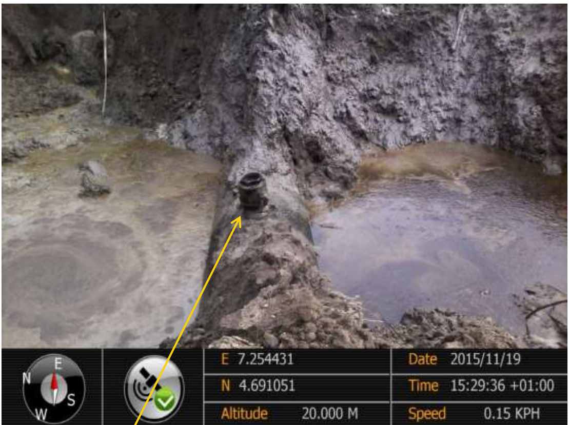
Close-up: Illegal fitting exposed on 28" Nkpoku – Bomu Pipeline at B-Dere. Picture was taken during Joint Investigation of 19 th November 2015.
