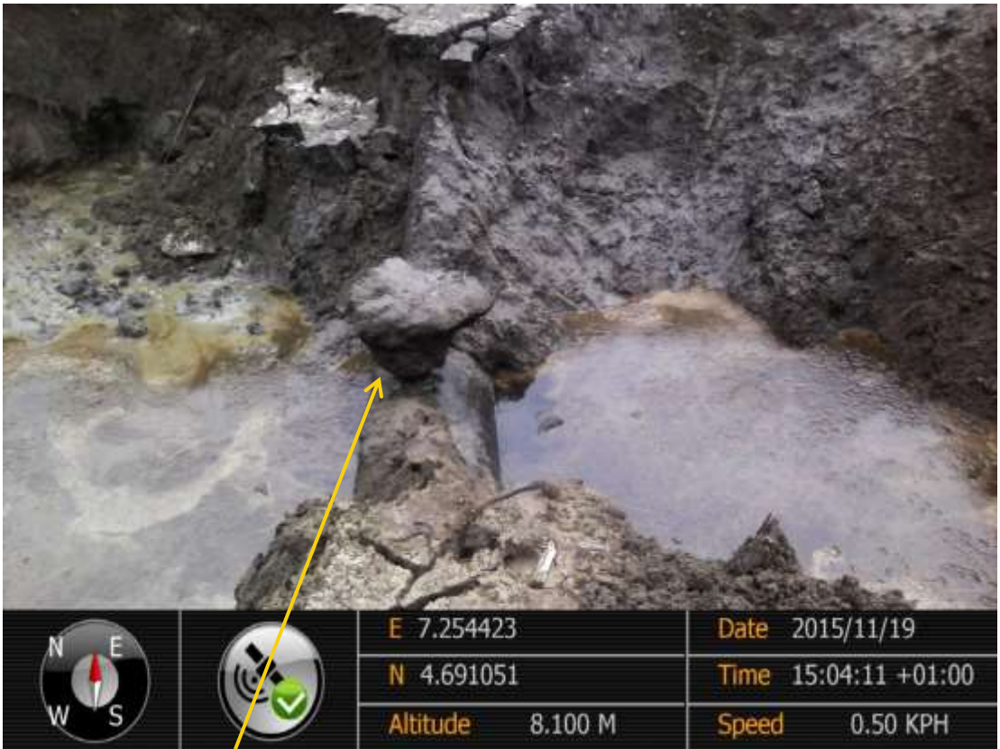
Close-up: Illegal fitting with concrete cap on 28" Nkpoku – Bomu Pipeline at B-Dere. Picture was taken during Joint Investigation of 19 th November 2015.
