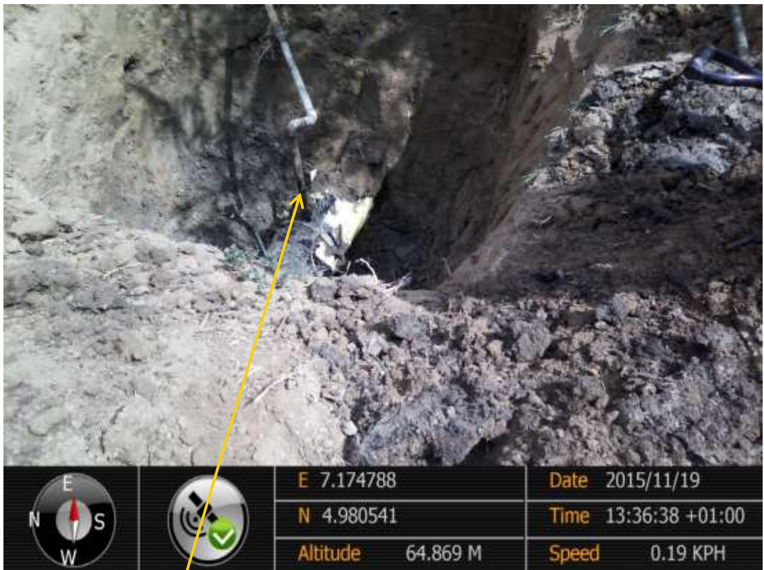
Close-up: Illegal fitting on 12" Imo River2 – Ogale Pipeline at Owaza. Picture was taken during Joint Investigation of 19 th November 2015.
