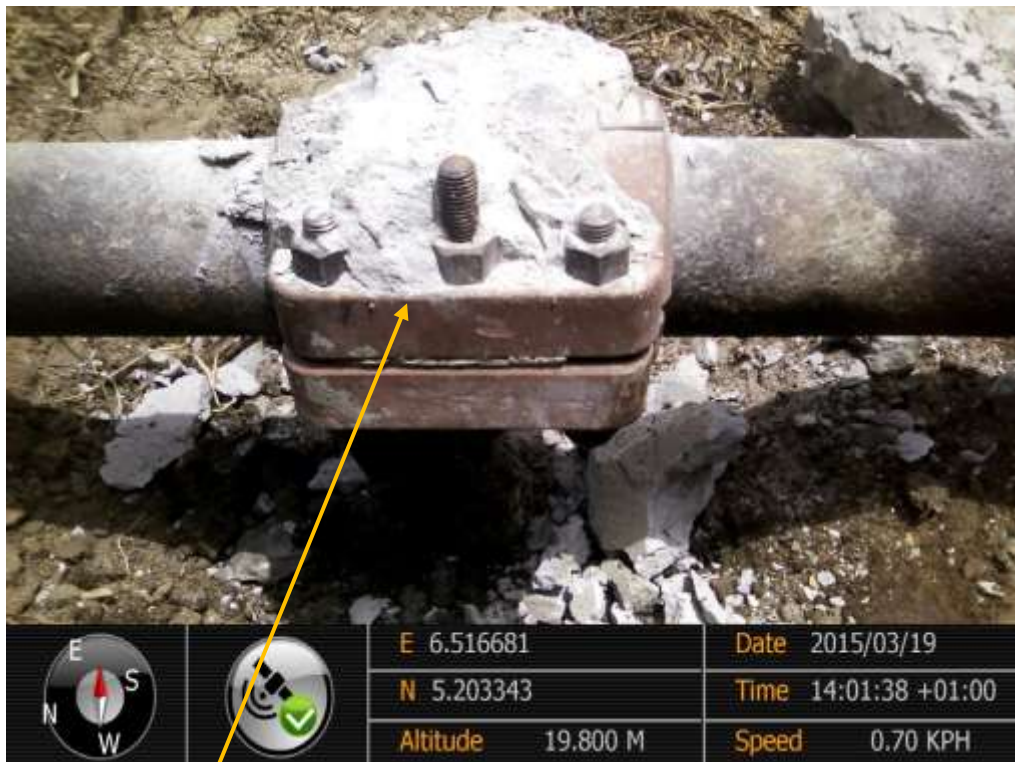
Close-up: Failed clamp on Adibawa Well10S Flowline at Edagberi/Betterland. Picture was taken during Joint Investigation of 19 th of March 2015.
