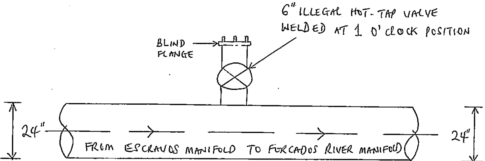
24" TRANS - ESCRAVOS PIPELINE AT SOKEBLOU
