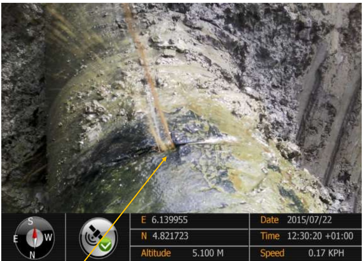
Close-up: Hacksaw cut on 16" NunRiver - KoloCreek Pipeline at Angiama. Picture was taken during Joint Investigation of 22nd July 2015.
