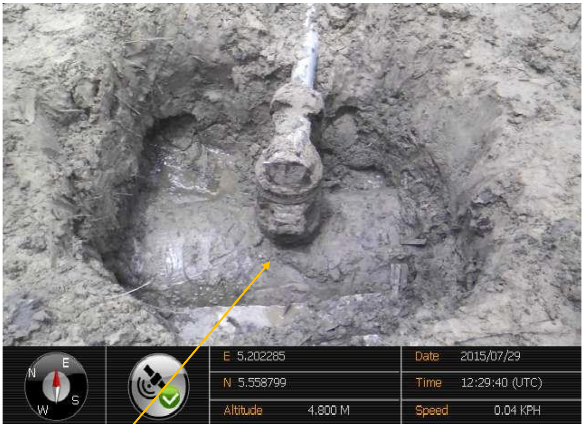
Close-up: Illegal fitting on 20" Otumara - Escravos Pipeline at Ogidigben. Picture was taken during Joint Investigation of 29 th July 2015.
