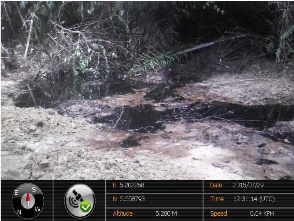
Overview: Part of spill impact on 20" Otumara - Escravos Pipeline at Ogidigben. Picture was taken during Joint Investigation of 29 th July 2015.
