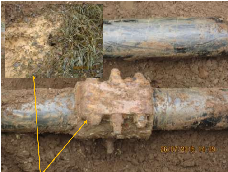
Close-up: Hole created by gas release and Failed clamp on Nkali Well 10L Flowline at Odagwa. Picture was taken during Joint Investigation of 26th July 2015.
