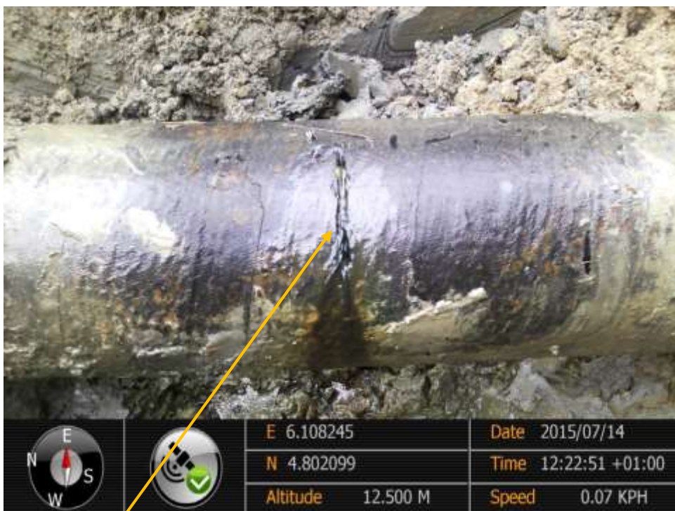
Close-up: Hacksaw cut (C) on 10" Diebu Creek – Nun River Pipeline at Oporoma. Picture was taken during Joint Investigation of 14 th July 2015.
