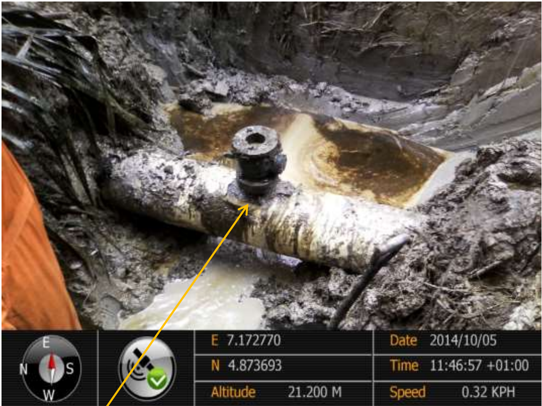
Close-up: Illegal fitting on 12" Imo River – Ogale Pipeline at KomKom. Picture was taken during Joint Investigation of 5 th October 2014.
