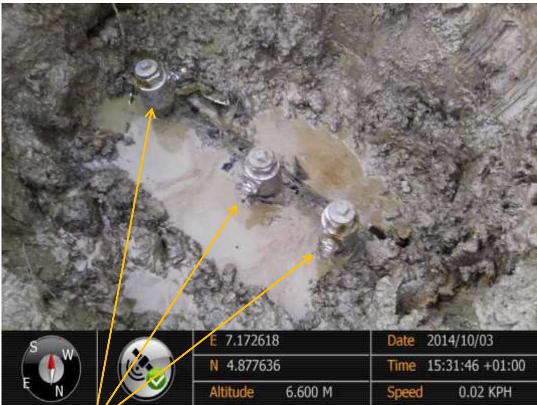
Close-up: Illegal fittings on 12" Imo River – Ogale Pipeline at KomKom. Picture was taken during Joint Investigation of 3 rd October 2014.
