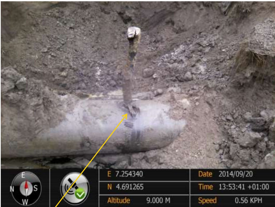
Close-up: Wooden plug at spill point on 28" Nkpoku-Bomu Pipeline at B-Dere. Picture was taken during Joint Investigation of 20 th September 2014.
